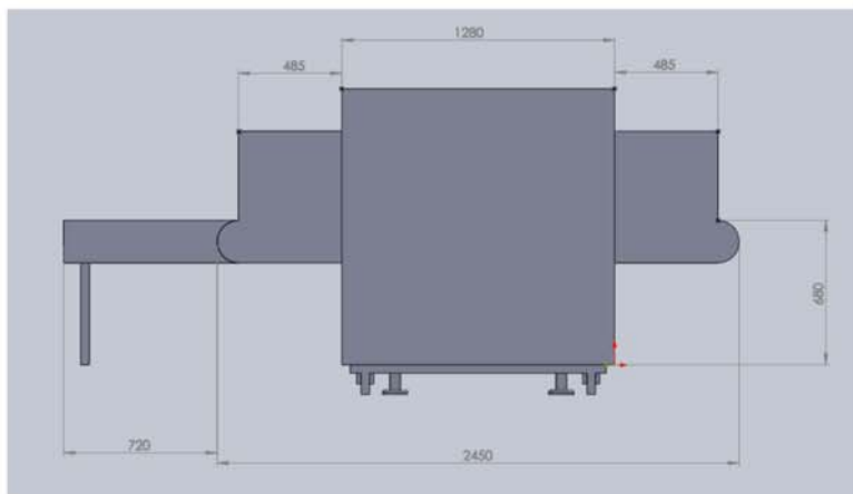
TR70 – Front View
