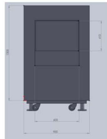
TR70 – Side View
